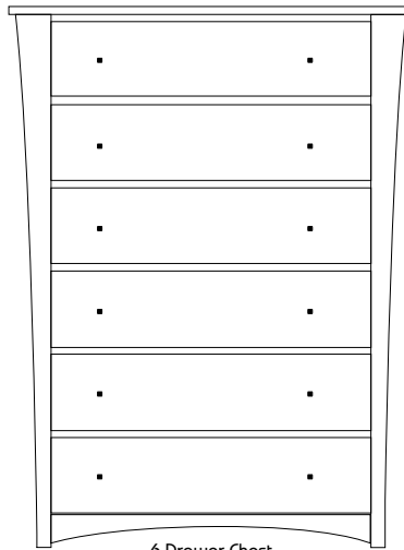
6 Drawer Chest 1230h x 860w x 475d
